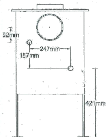
Positions of boiler pipes
